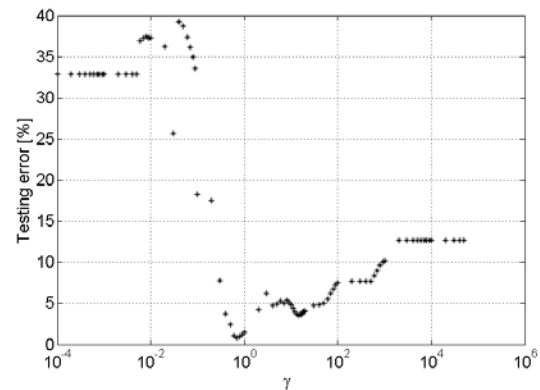
Fig. 6 Example of influence of coefficient \gamma on testing error.
